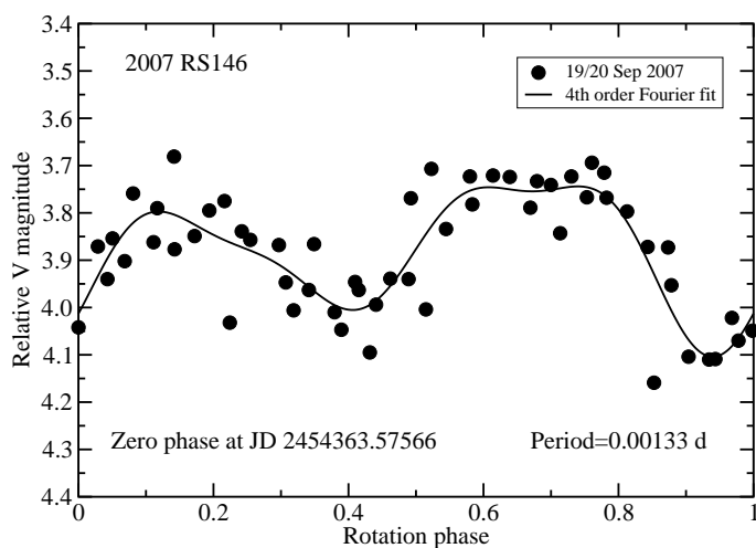
Fig. 12. Composite lightcurve of 2007 RS 146 obtained with a period of P_1 = 0.03209 \pm 0.00004 h.
