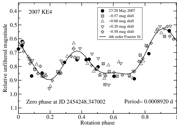
Fig. 9. Composite lightcurve of 2007 KE4 obtained with a period of P = 0.021408 \pm 0.000007 h
