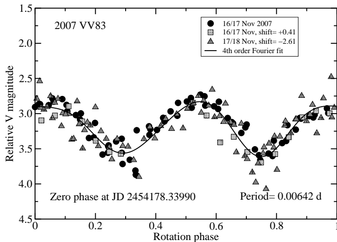
Fig. 14. Composite lightcurve of 2007 VV83 obtained with a period of P = 0.15392 \pm 0.00045 h.
