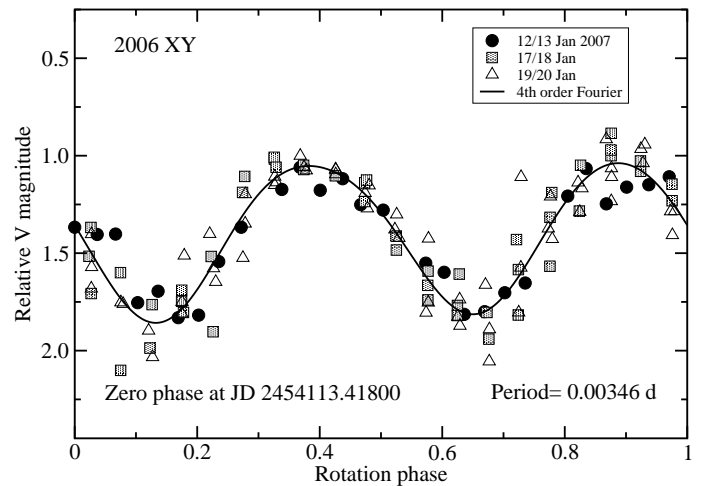
Fig. 4. Composite lightcurve of 2006 XY, obtained with a period of 0.0832 \pm 0.0001 h.
