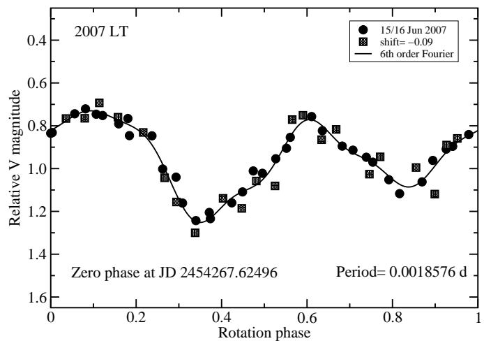
Fig. 10. Composite lightcurve of 2007 LT obtained with a period of P = 0.044583 \pm 0.000022 h
